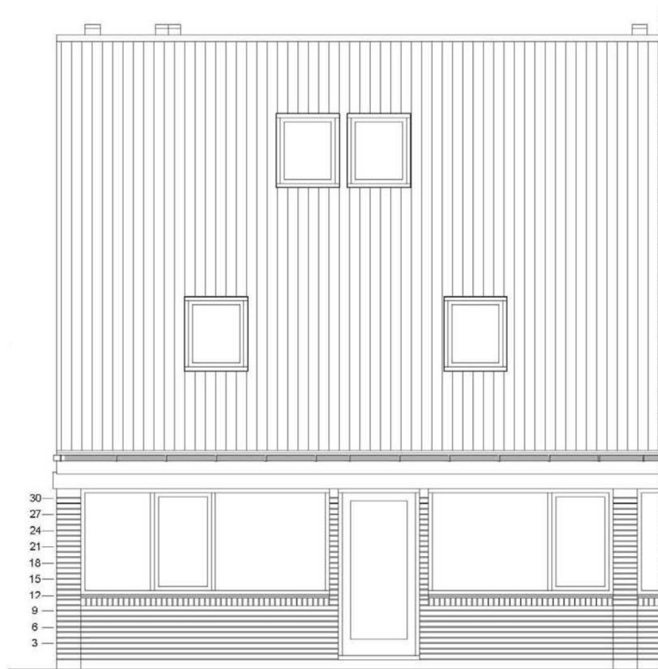
Facade Vest
